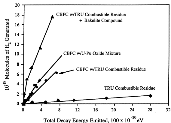
Fig. 6. Molecules of H 2 generated by radiolysis for the three Pu-laden CBPC samples and a sample of TRU combustible residue.
