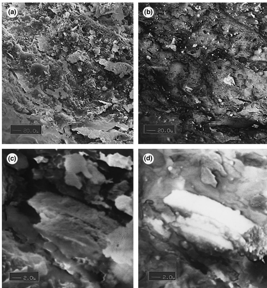
Fig. 5. SEM photomicrographs of fractured surface of waste form of combustion residue without organics: (a) direct image at low magnification, (b) back-scattered image at low magnification, (c) direct image at high magnification, and (d) back-scattered image at high magnification.
