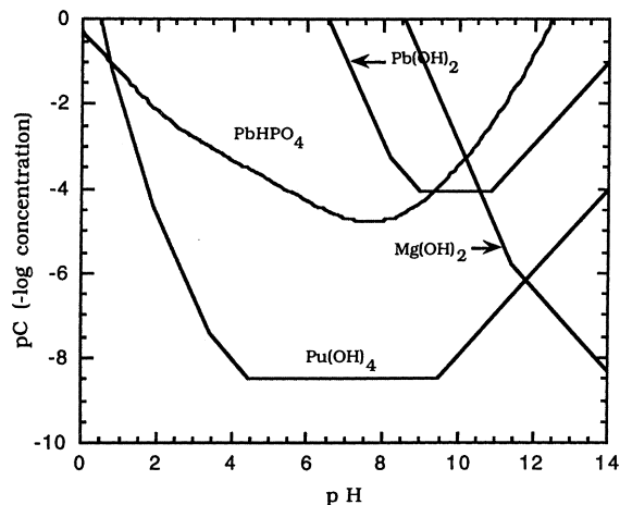
Fig. 8. Dissolution characteristics of Pu, Pb, and Mg in acid-base reaction of CBPC process.
