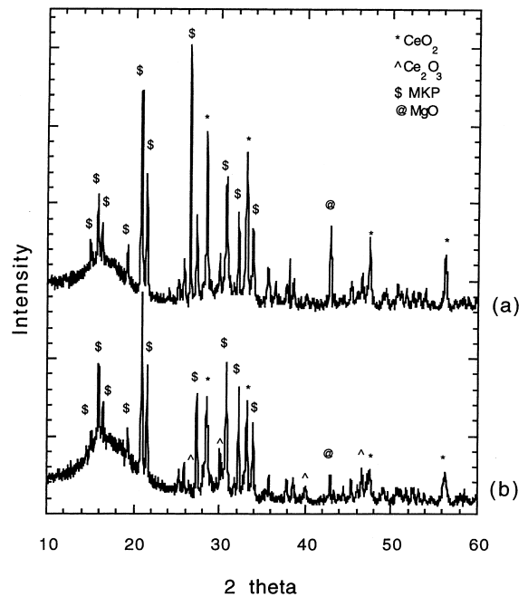
Fig. 2. X-ray diffraction patterns of waste forms containing (a) CeO 2 , and (b) Ce 2 O 3 as surrogates of PuO 2 and Pu 2 O 3 .
