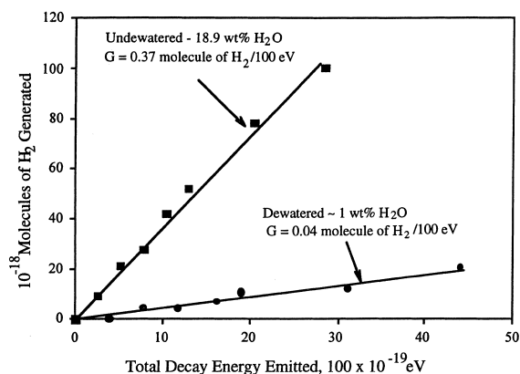
Fig. 7. Effect of water content on the rate of radiolytic \text{H}_2 generation for a Pu-laden CBPC sample. Dewatering was accomplished by heating a sample of the Pu-laden CBPC at 110 \pm 5^\circ\text{C} . for 1 h in a nitrogen atmosphere.
